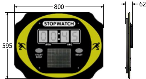
FISTOPWATCH6-D
